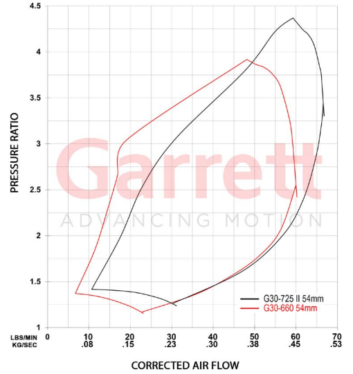
G30-725 Compressor Overlay
